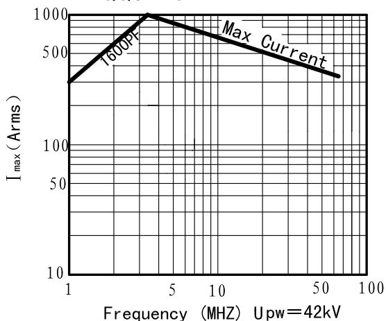
CONTINUOUS RMS AMPERES vs FREQUENCY
